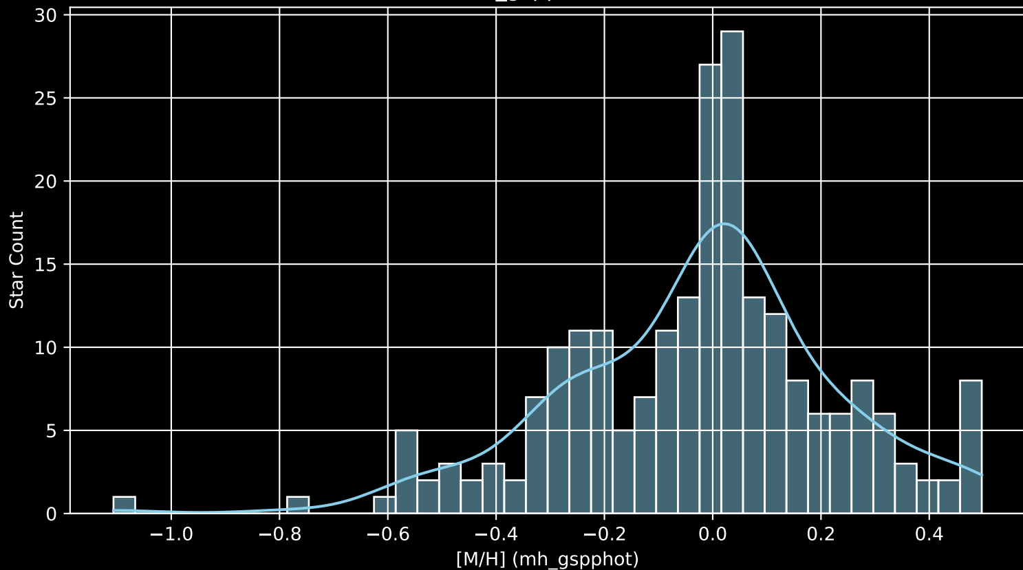
APOGEE DR17 Field: [M67-S [M/H] (mh_gspphot) (n= 225)
