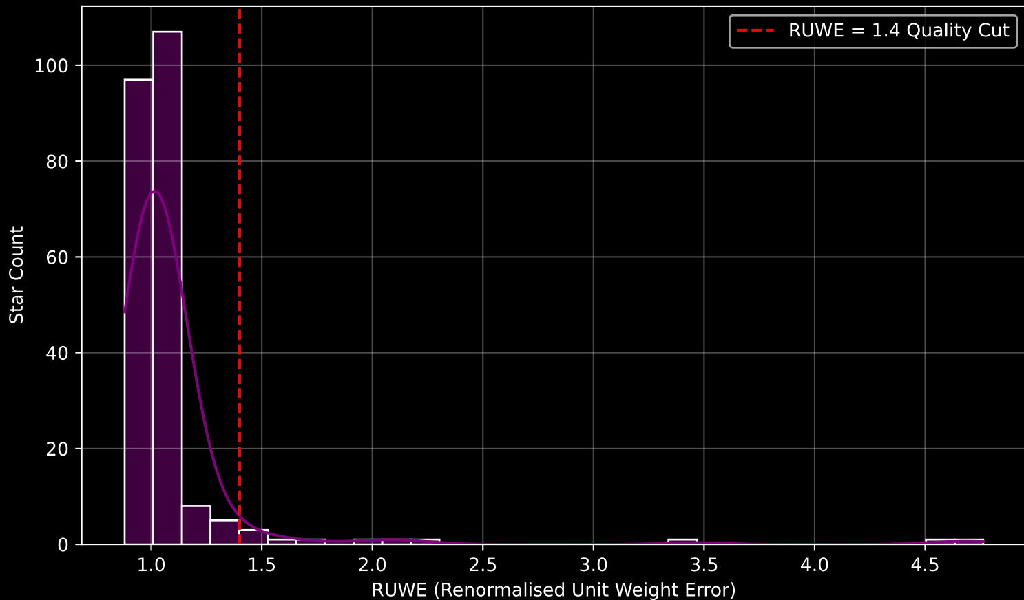
GAPOGEE DR17 Field [M67-S] RUWE Distribution (n= 228)
