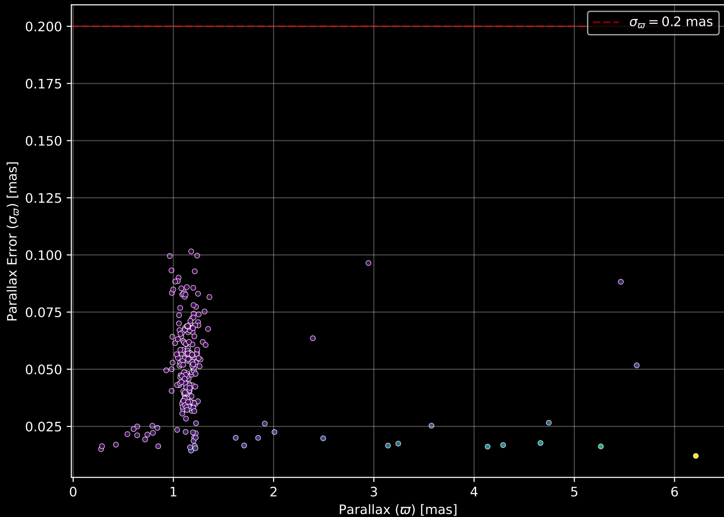
APOGEE DR17 Field: [M67-S] Parallax Quality (n= 229)
