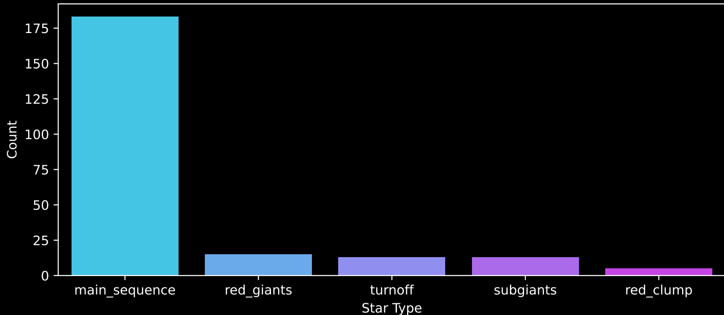
APOGEE DR17 Field: [M67-S] Count plot of Star Type
