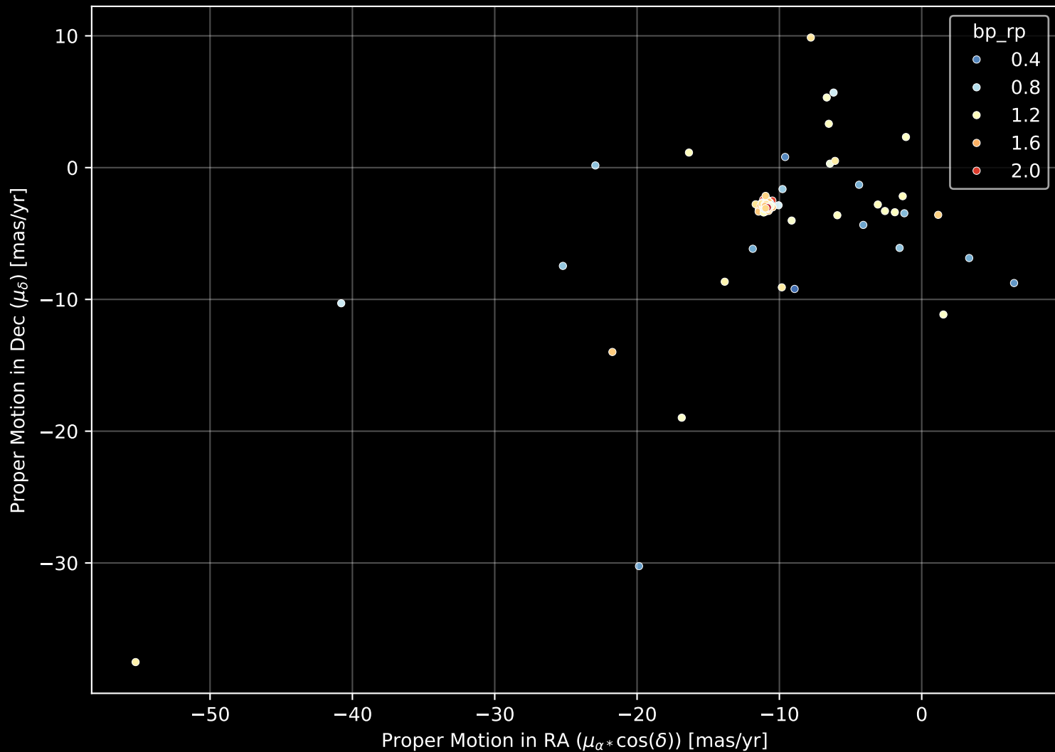
APOGEE DR17 Field: [M67-S] Proper Motion Diagram (n= 229)
